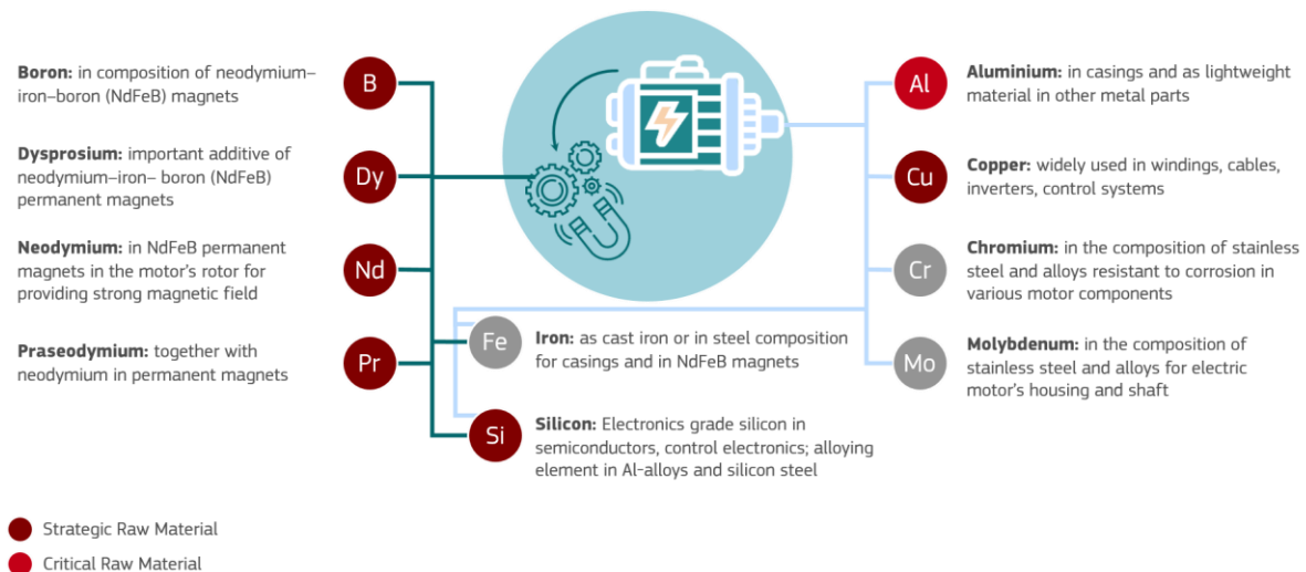
Figure 36. Selection of raw materials used in traction motors and their function
