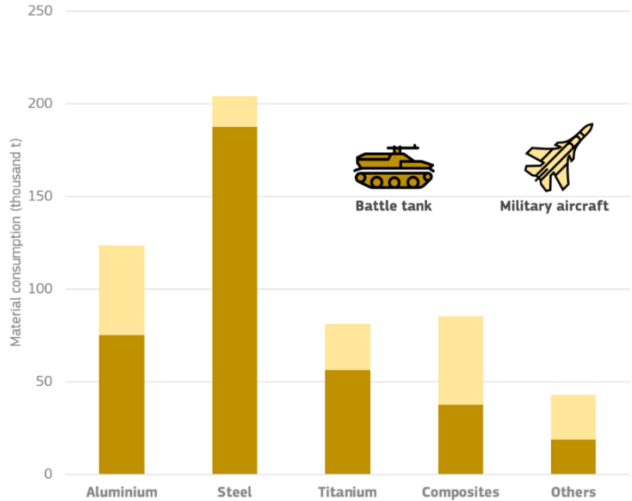
Figure 107. Demand for structural materials in NATO fleets of aircrafts and battle tanks as of 2022 74 .
