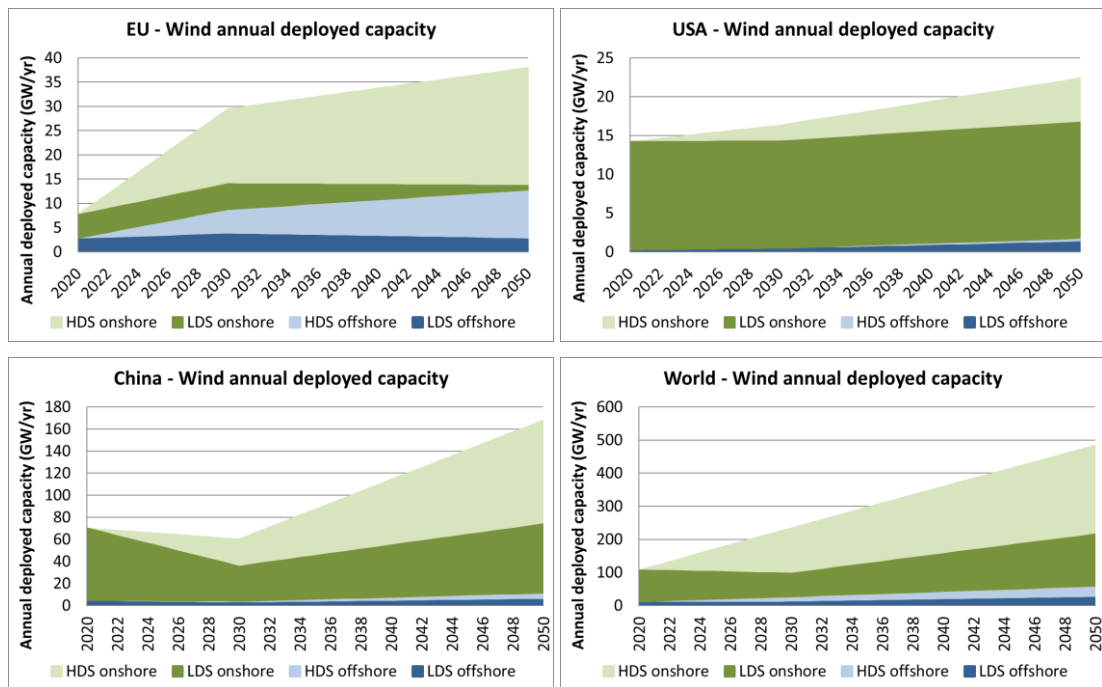
Figure 34. Onshore and offshore wind annual deployed capacity in the EU, US, China, and globally in the two explored scenarios
