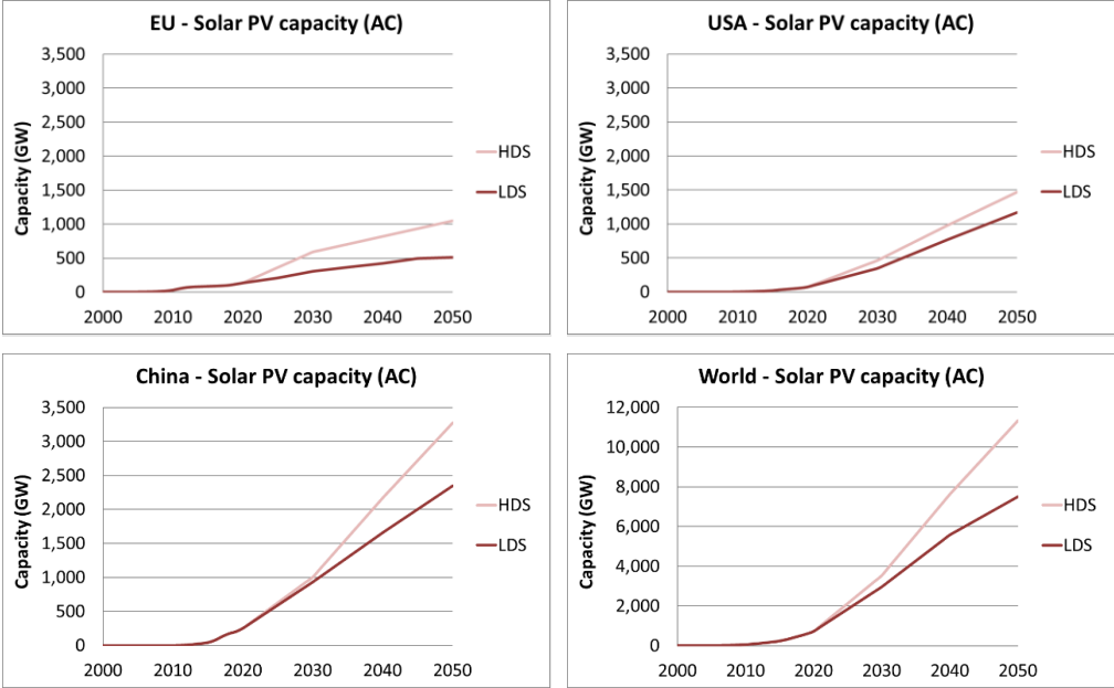
Figure 43. Solar PV capacity in the EU, US, China, and globally in the two explored scenarios
