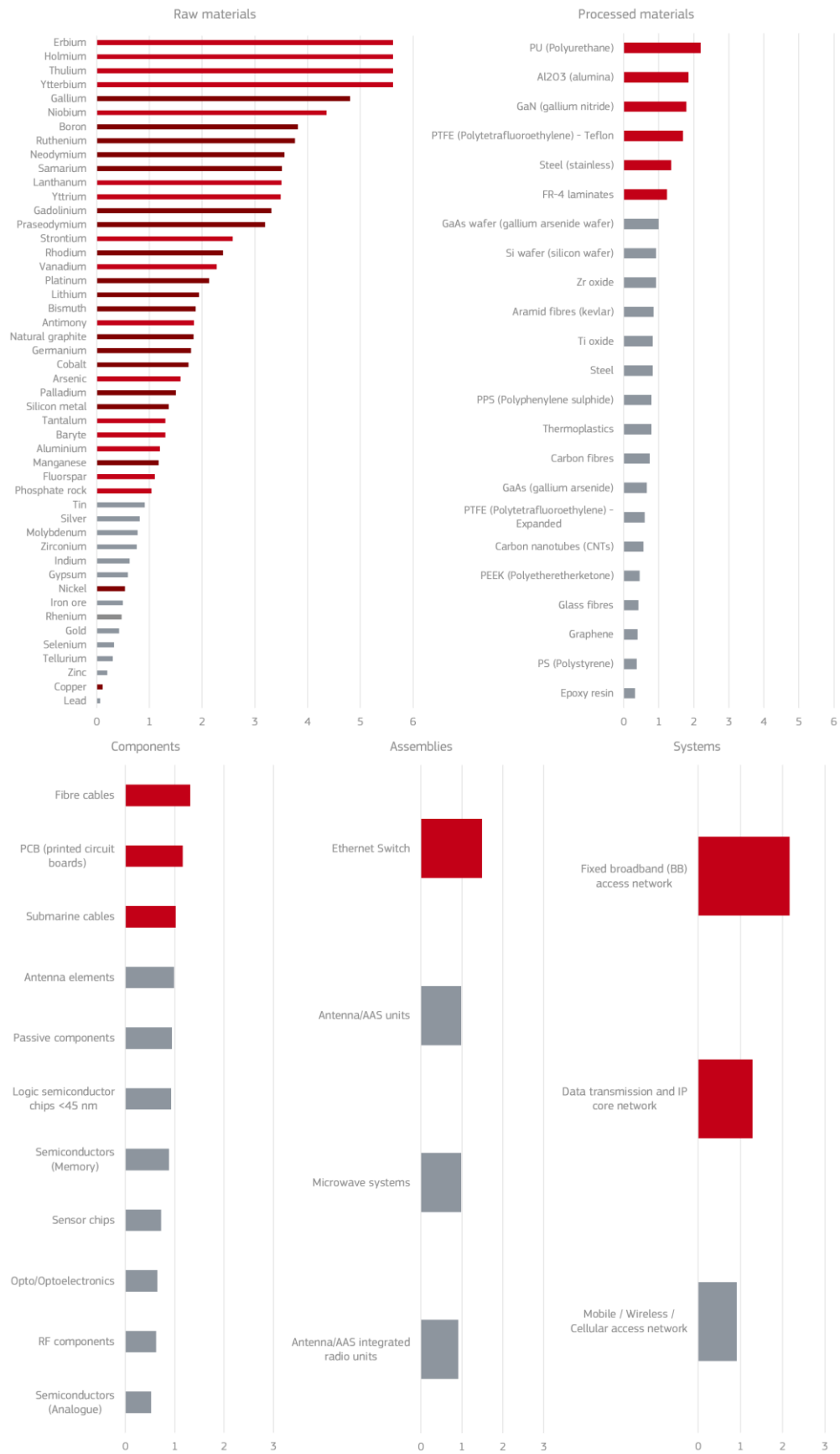
Figure 57. Detailed Supply Risk of selected elements in the data transmission networks supply chain
