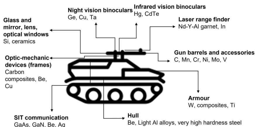
Figure 108. Components and raw materials used in a main battle tank (e.g. Leclerc), but also representative of infantry-fighting and armoured fighting vehicles
