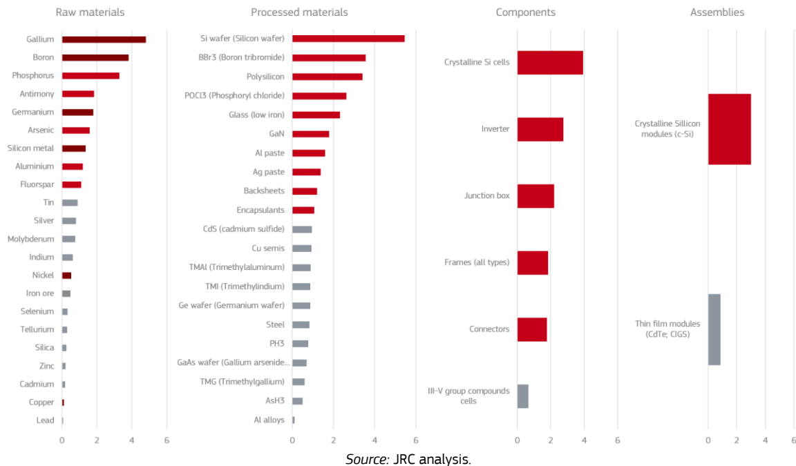
Figure 42. Detailed Supply Risk of selected elements in the Solar PV supply chain
