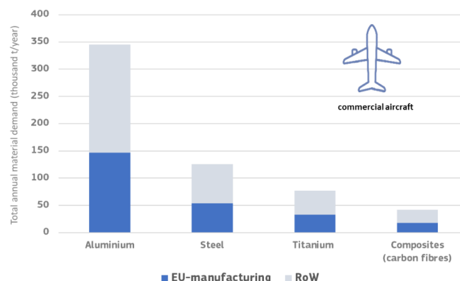
Figure 106. Total annual material demand in 2018 for commercial aircraft manufacturing (expressed in ktonnes per year). The figures includes manufacturing production losses.
