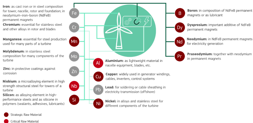
Figure 30. Selection of raw materials used in wind turbines and their function
