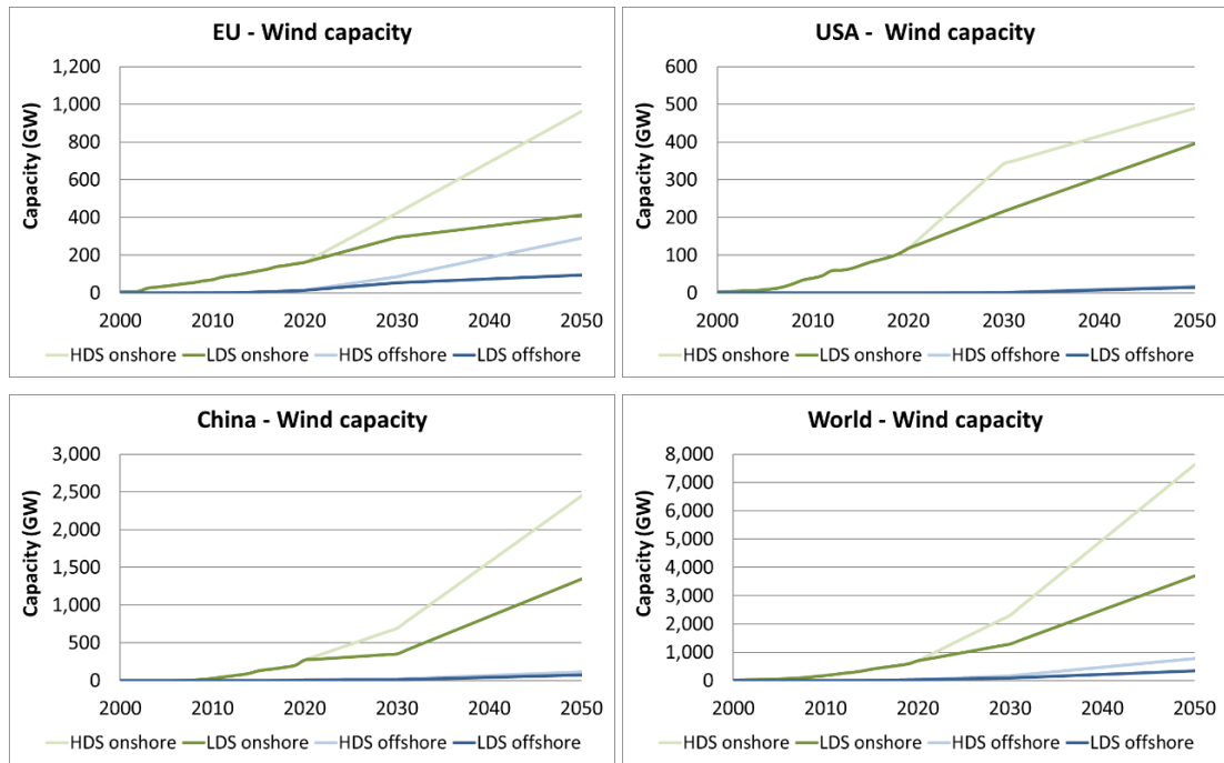
Figure 33. Onshore and offshore wind capacity in the EU, US, China, and globally in the two explored scenarios
