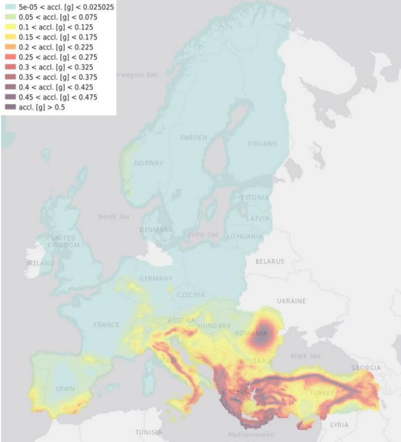
Figure 8. European seismic hazard map (mean values of PGA on reference rock with a return period of 475 years)
